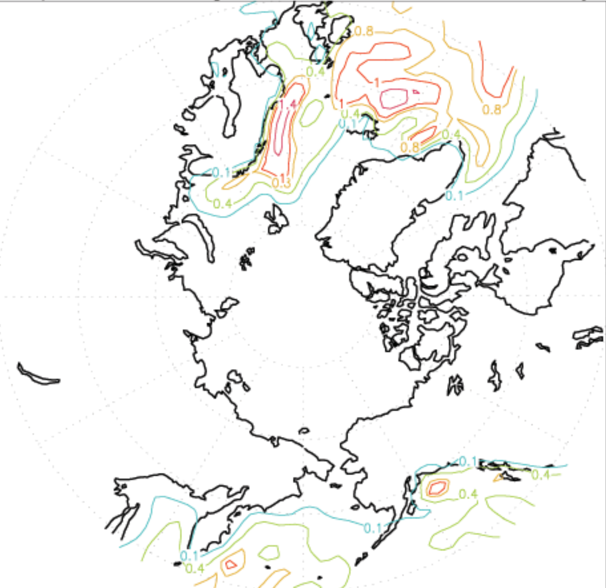
Deep convective heating rate, 1950-2002, ~800 hPa, DJF, Kday -1
